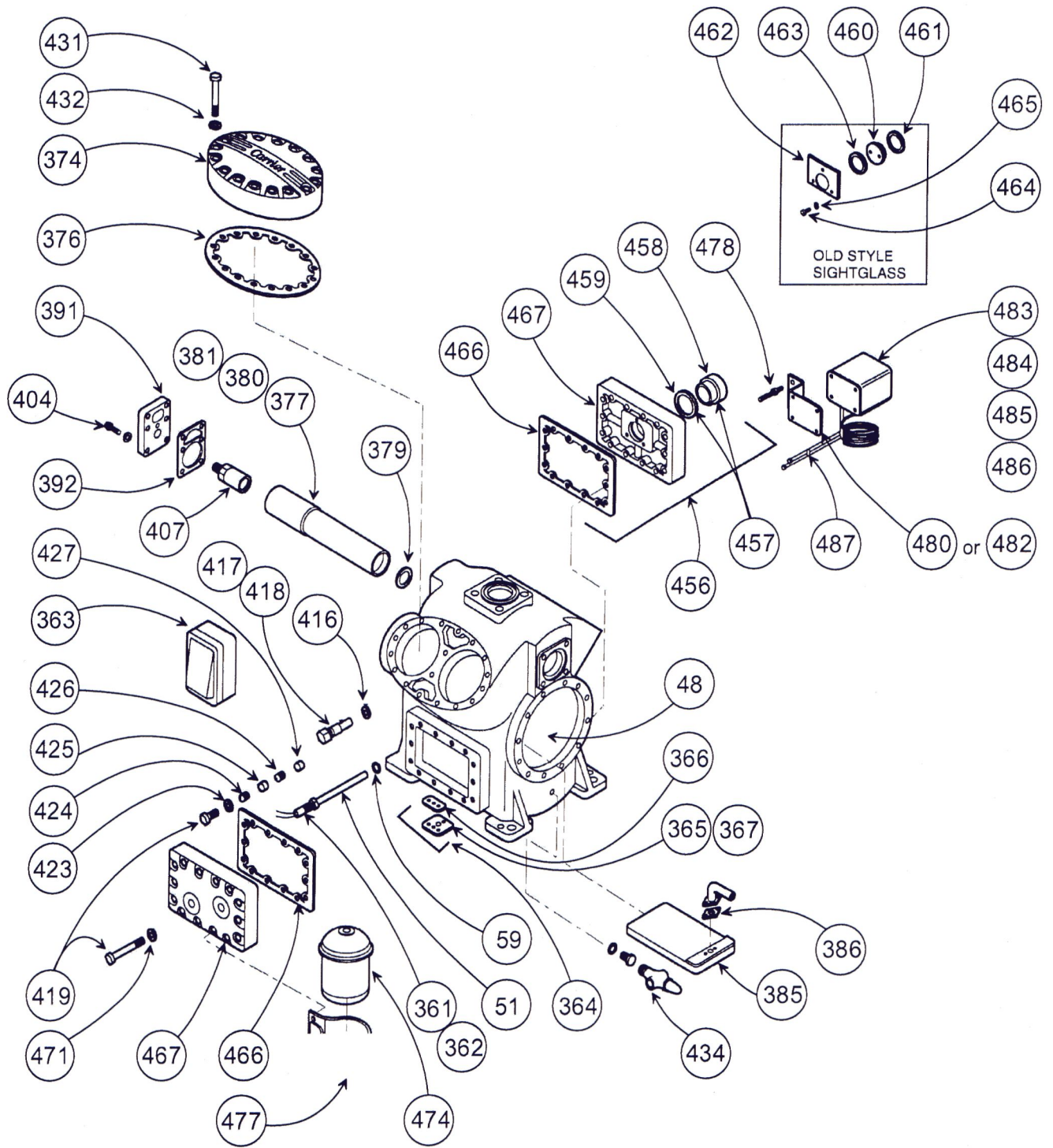
5H40.46 SHOWN
